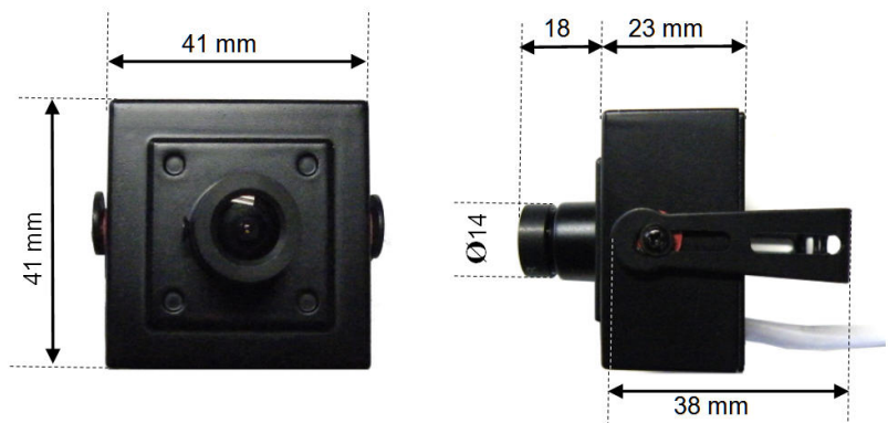
Cable length 60 cm No connector on the camera rear face
